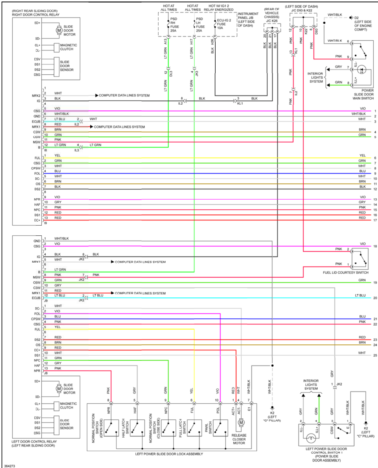
Fig. 120: Power Sliding Door Circuit (1 of 3)
