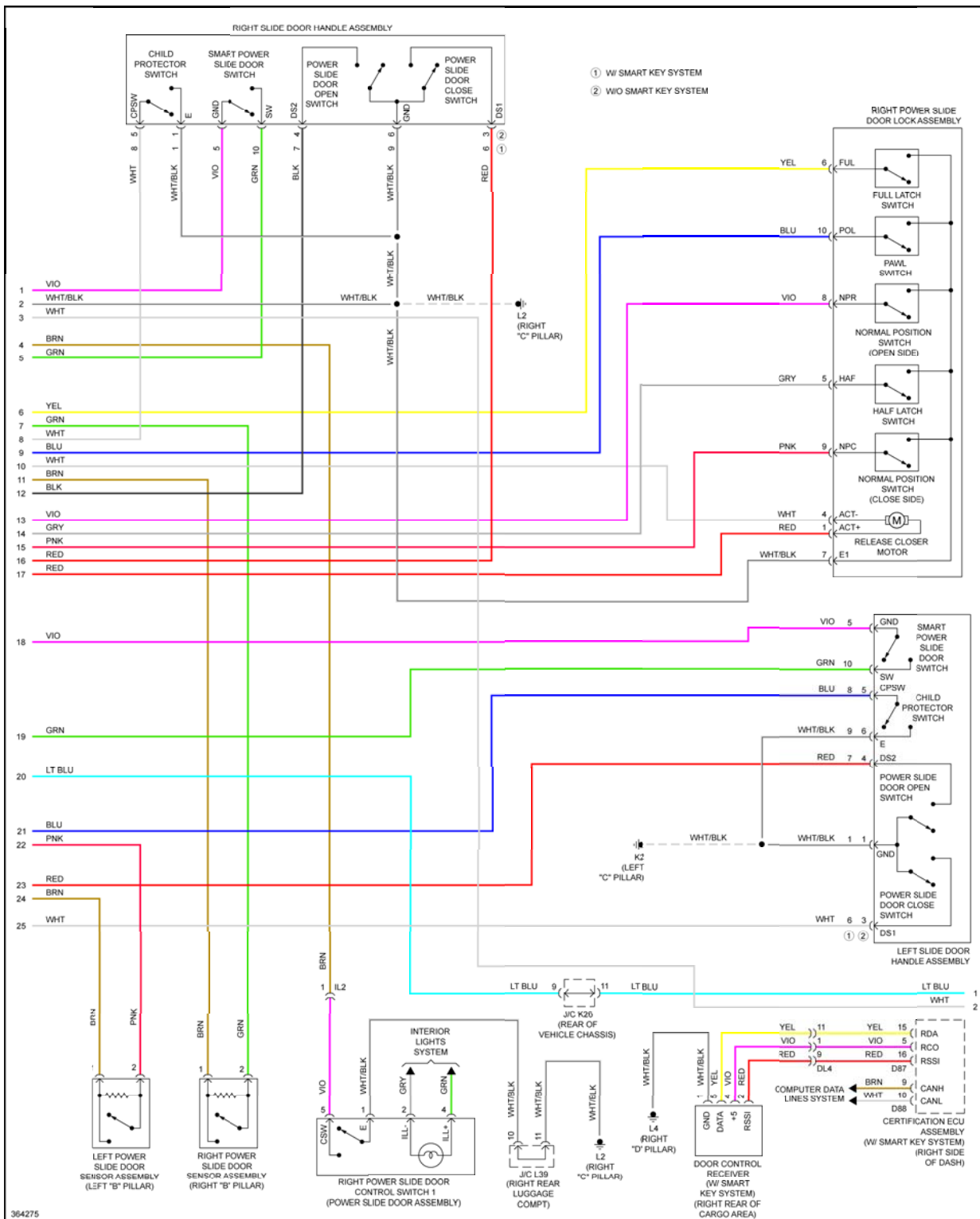
Fig. 121: Power Sliding Door Circuit (2 of 3)
