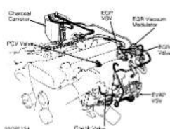
Fig. 24: Vacuum Diagram (Supra Turbo) Courtesy of Toyota Motor Sales, U.S.A., Inc.
