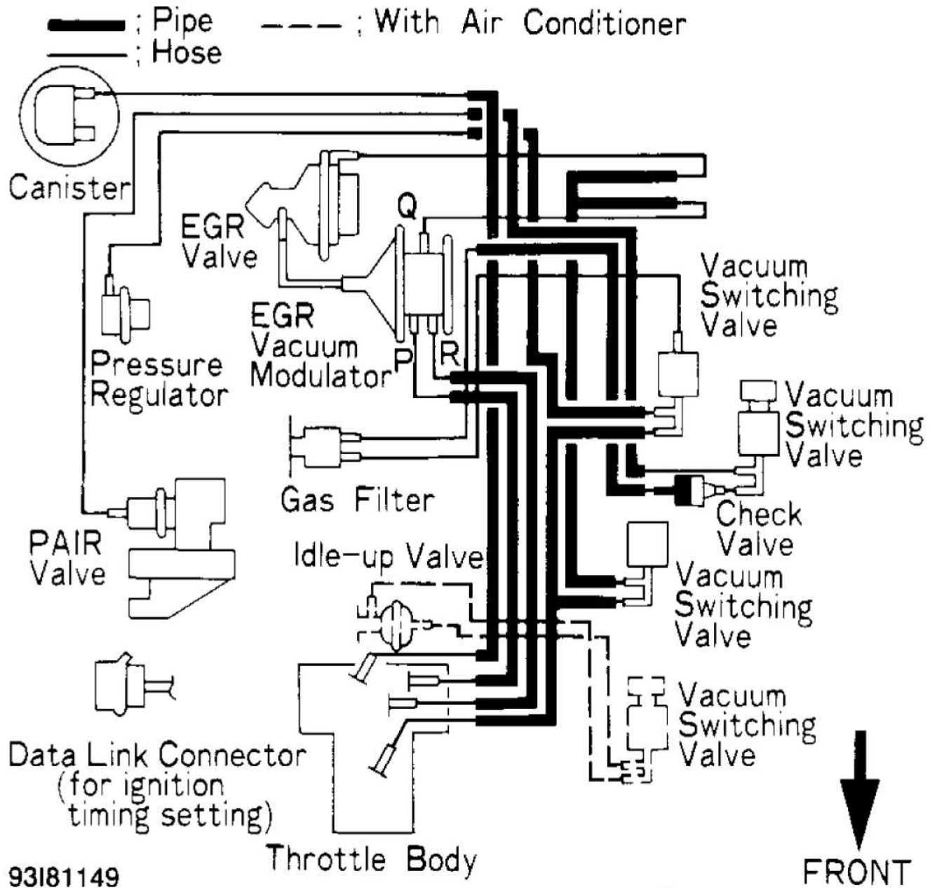
Fig. 19: Vacuum Diagram (Pickup 2.4L &amp; 4Runner 2.4L - California M/T)
