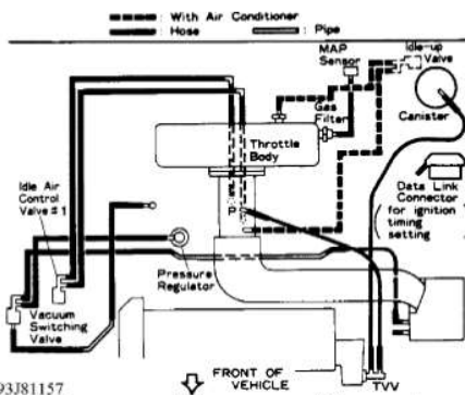
Fig. 27: Vacuum Diagram (Tercel - Federal Models W/O Power Steering) Courtesy of Toyota Motor Sales, U.S.A., Inc.
