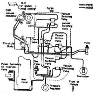
Fig. 10: Vacuum Diagram (Land Cruiser) Courtesy of Toyota Motor Sales, U.S.A., Inc.
