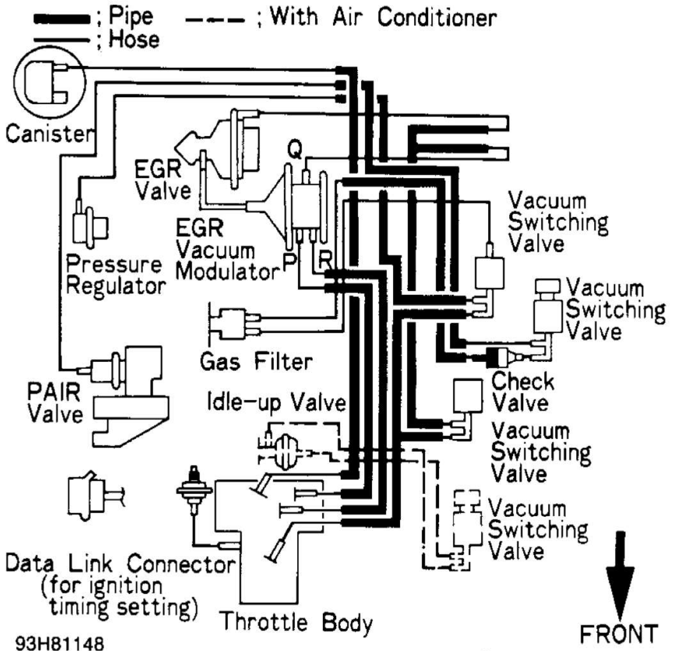
Fig. 18: Vacuum Diagram (Pickup 2.4L &amp; 4Runner 2.4L - California A/T)
