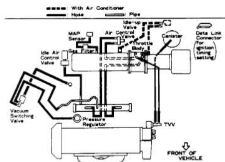
Fig. 15: Vacuum Diagram (Paseo - California Models) Courtesy of Toyota Motor Sales, U.S.A., Inc.
