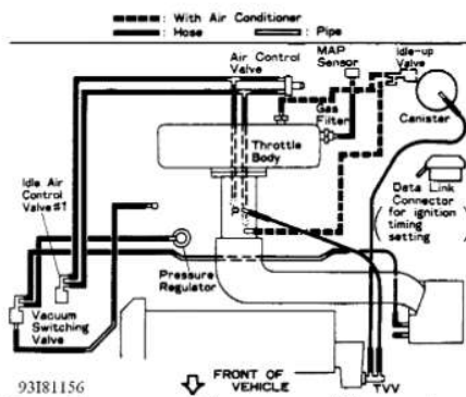
Fig. 26: Vacuum Diagram (Tercel - Federal Models W/ Power Steering) Courtesy of Toyota Motor Sales, U.S.A., Inc.
