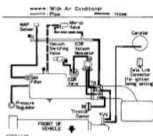
Fig. 9: Vacuum Diagram (Corolla - Calif. Models W/O Power Steering) Courtesy of Toyota Motor Sales, U.S.A., Inc.
