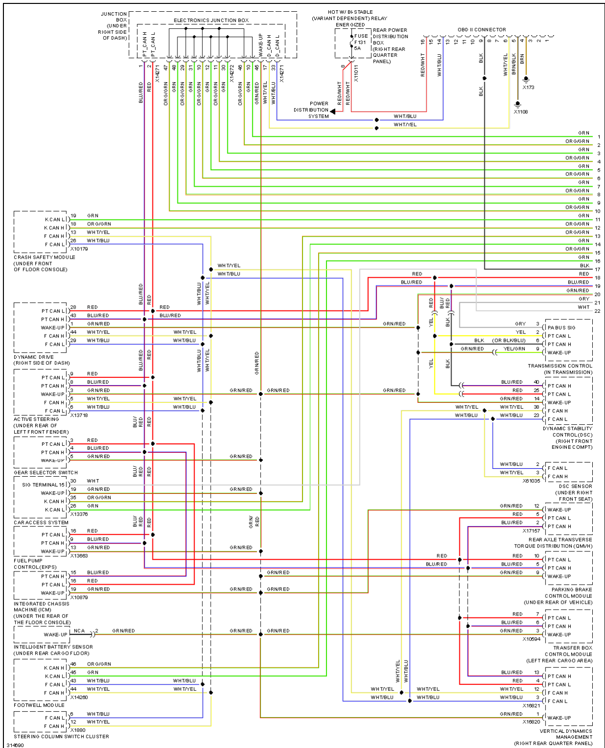
Fig. 19: Computer Data Lines Circuit (1 of 2)
