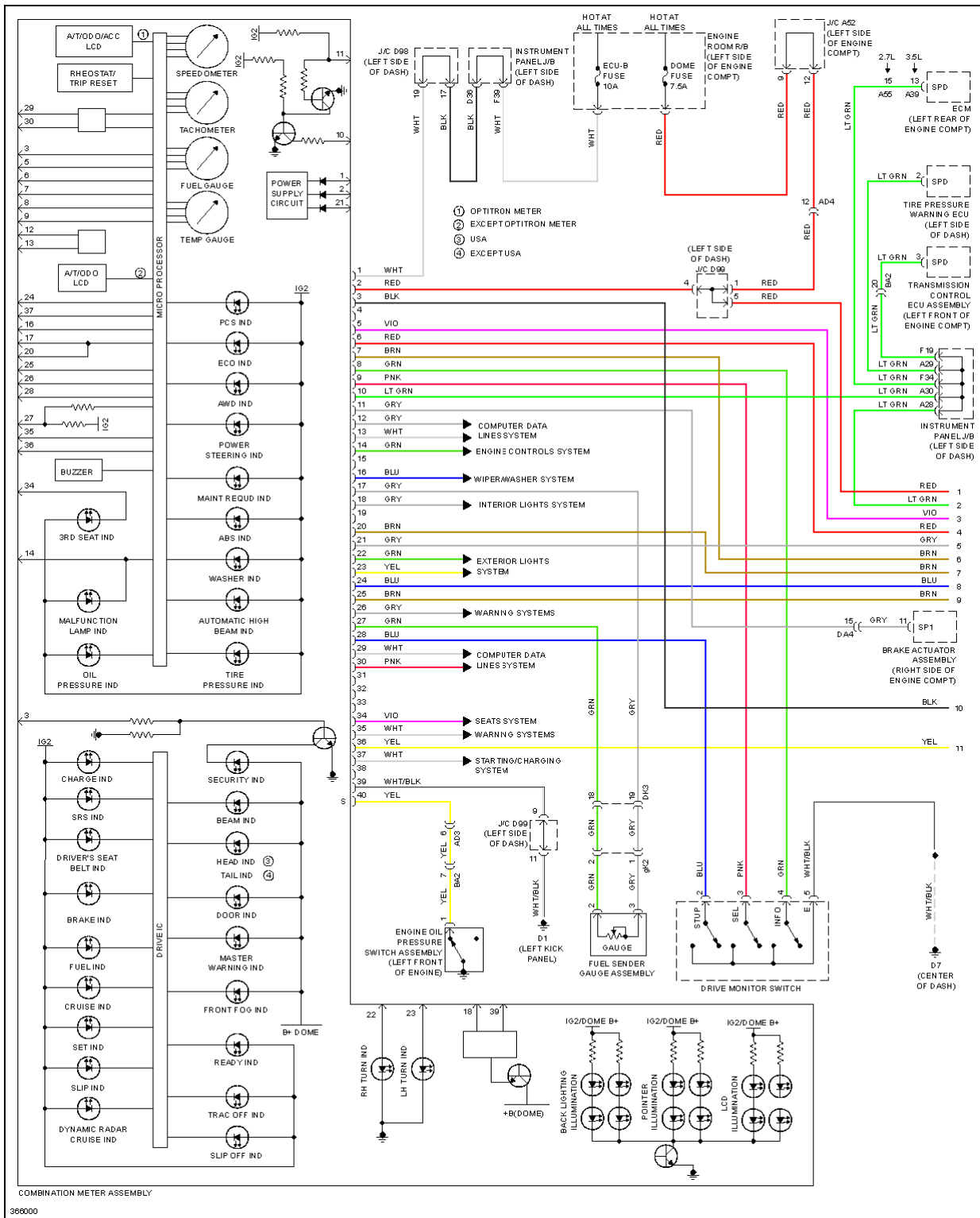
Fig. 51: Instrument Cluster Circuit (1 of 2)
