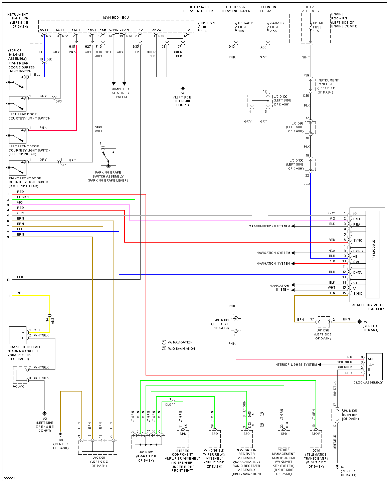
Fig. 52: Instrument Cluster Circuit (2 of 2)
