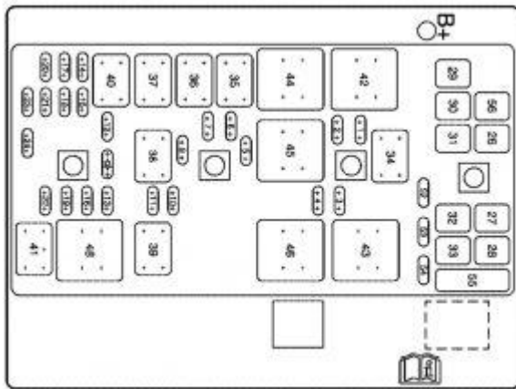
Pontiac Grand Prix mk7 – fuse box – engine compartment (3.8 engine)
