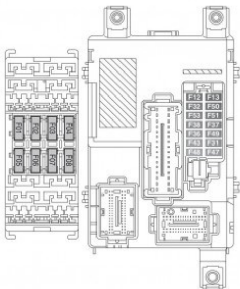
Fiat Doblo Panorama – fuse box – passenger compartment
