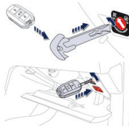
Passenger airbag OFF
