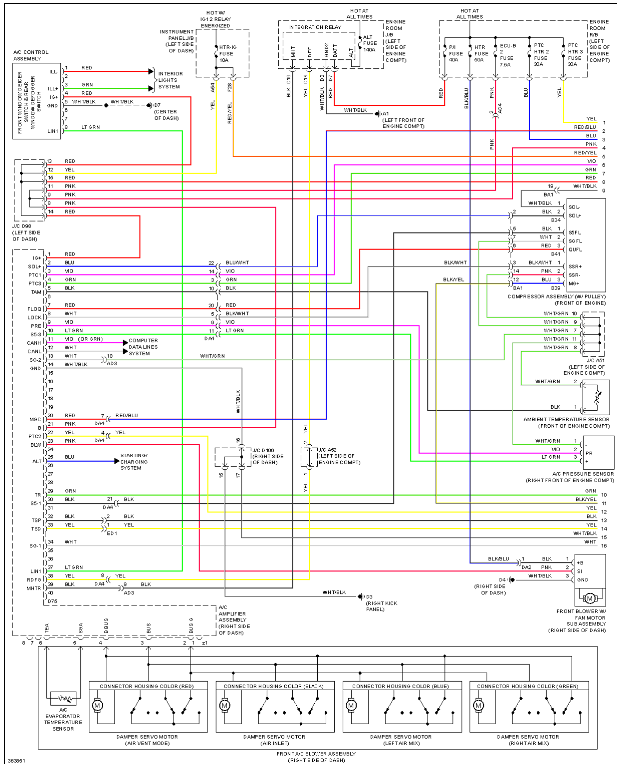
Fig. 1: A/C Circuit (1 of 2)
