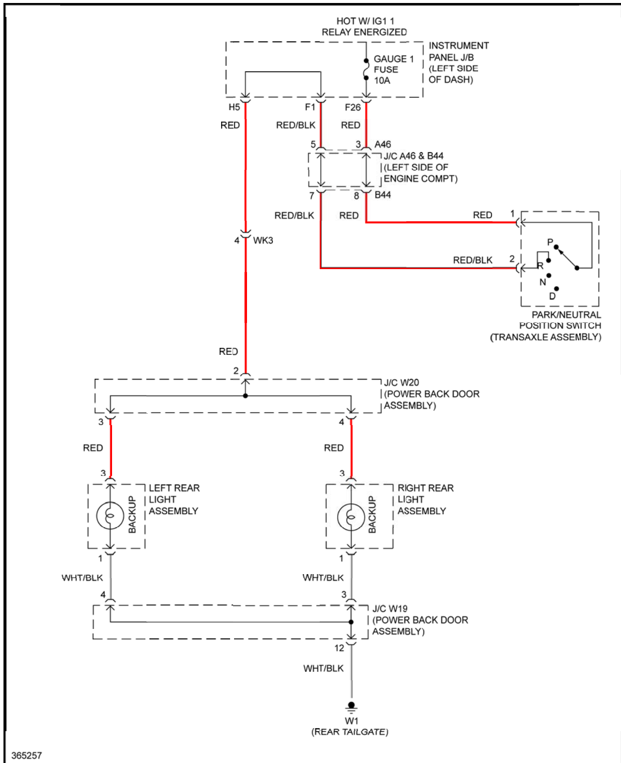
Fig. 39: Backup Lamps Circuit
