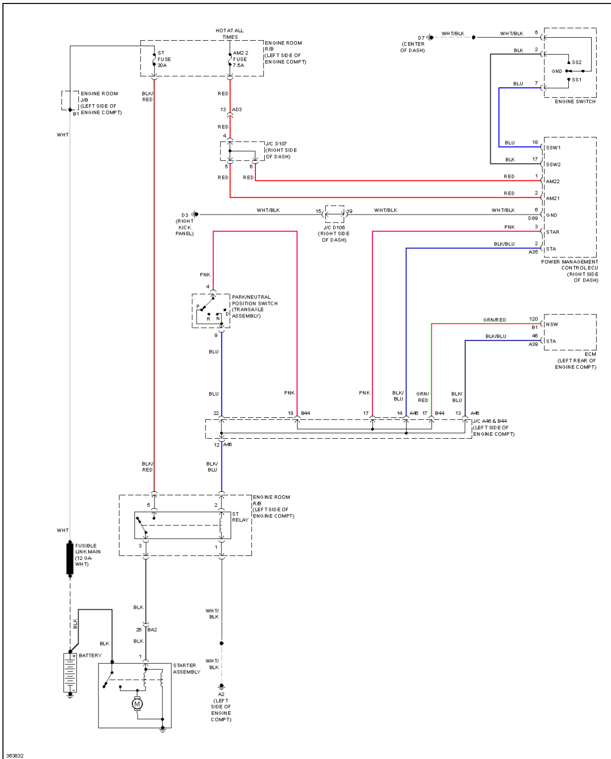
Fig. 106: Starting Circuit, W/ Smart Key System
