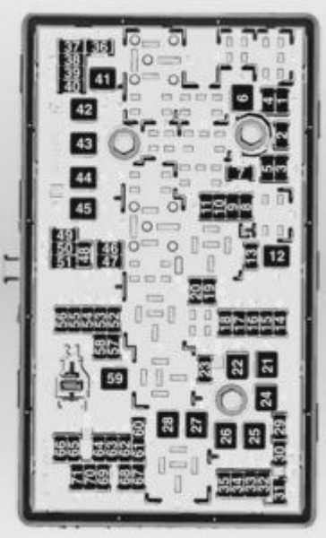
Chevrolet Cruze Station Wagon – fuse box – engine compartment
