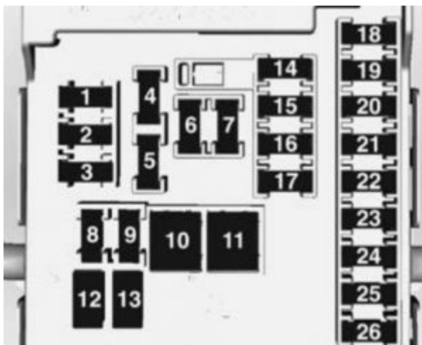
Chevrolet Cruze Station Wagon – fuse box –
