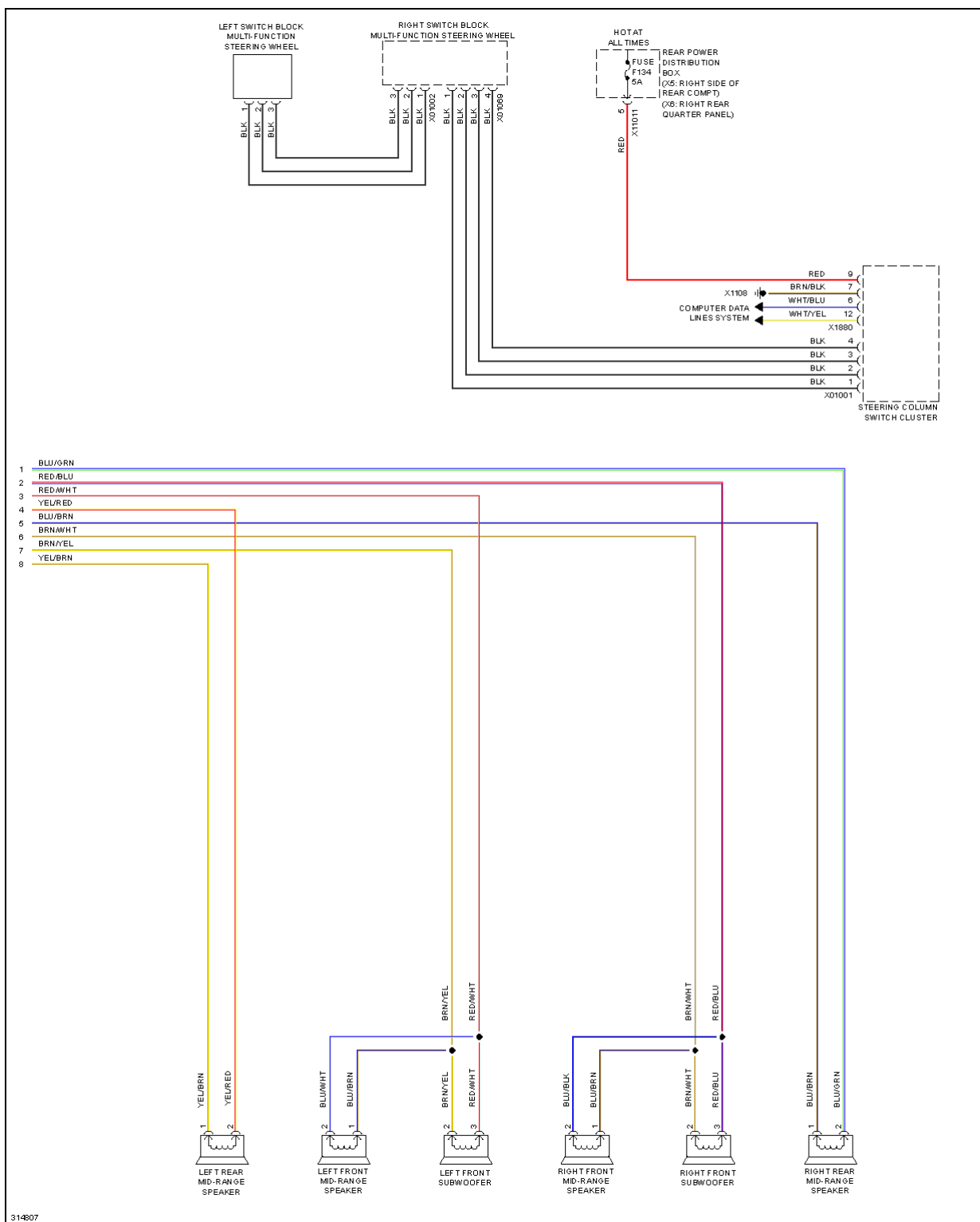
Fig. 106: Radio Circuit, W/ CCC & M-ASK (3 of 3)
