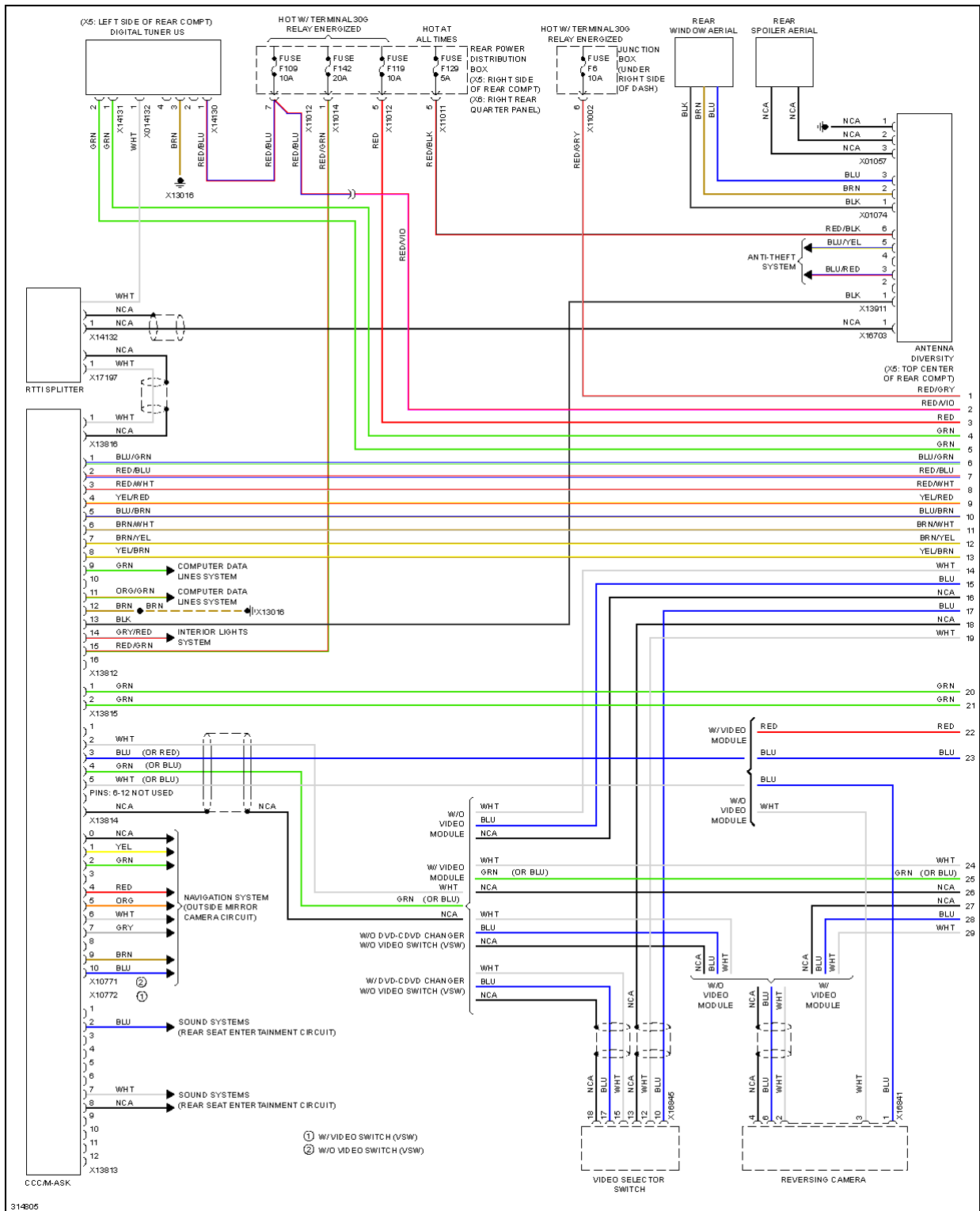
Fig. 104: Radio Circuit, W/ CCC & M-ASK (1 of 3)
