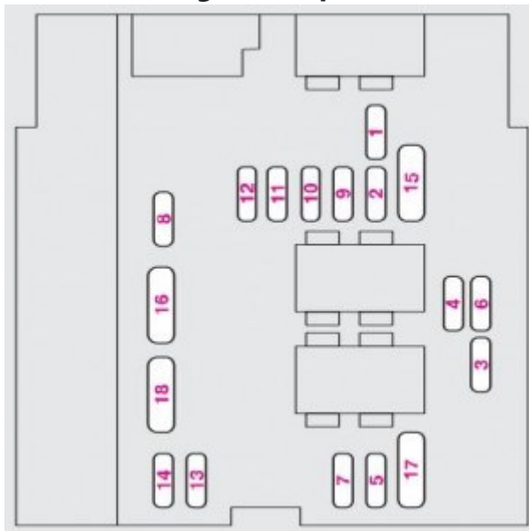
Fiat Ulysse mk2 – fuse box – engine compartment
