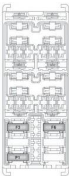
Alfa Romeo MiTo FL – fuse box – luggage
