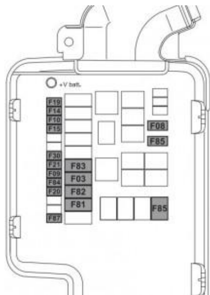
Alfa Romeo MiTo FL – fuse box – engine
