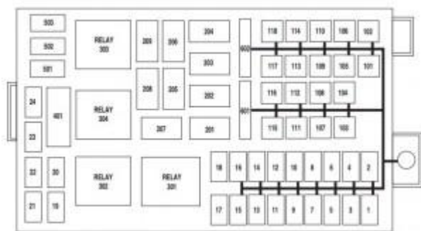
Merucry Monterey – fuse box – power distribution box
