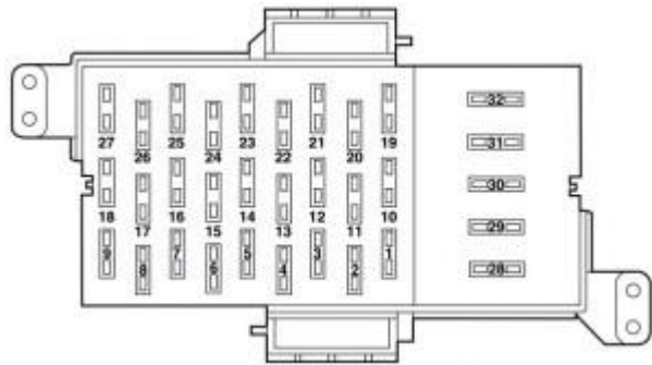
Merucry Monterey – fuse box – passenger compartment
