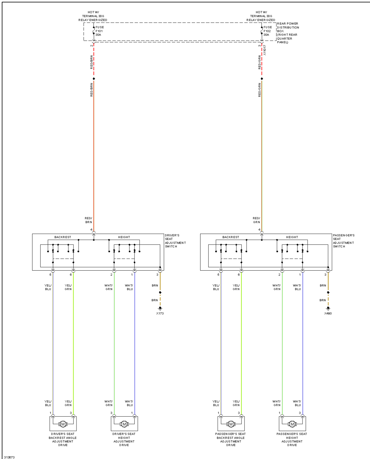
Fig. 95: Power Seats Circuit, W/ Driver & Passenger Power Seats
